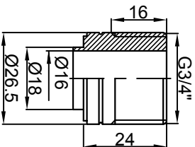
G3/4"Connection(L011D) F3 F4
